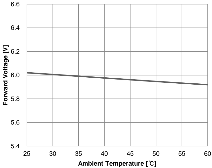
Fig 7. Ambient Temperature vs. Forward Voltage, I_F=200mA
