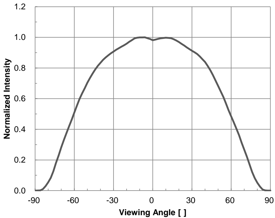
Fig 8. Typical Spatial Distribution, I_F=200mA
